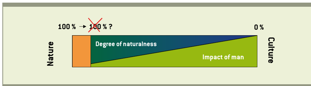
Figure 10. Theory of the naturalness gradient (modified from Winter et al. 2010).
