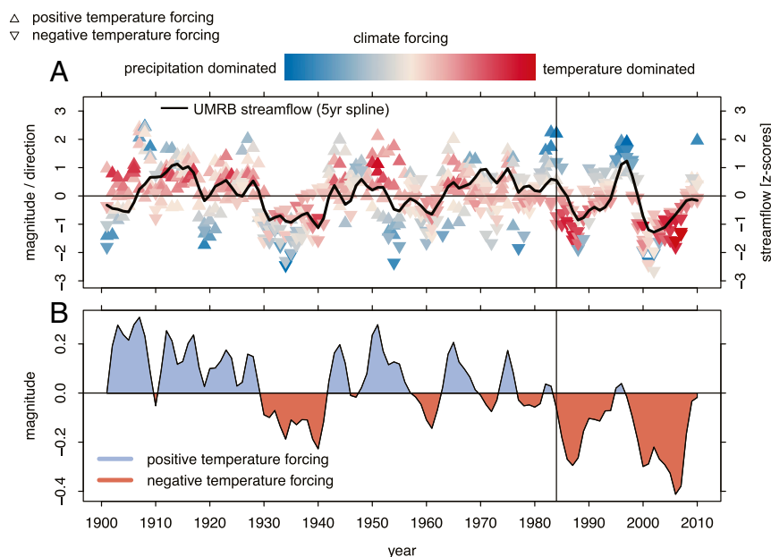
Fig. 3. Climate forcing of streamflow. (A) The relative forcing of precipitation and temperature (arrows) on basin-wide mean annual streamflow (black line) in the UMRB. Colored arrows show the individual relative forcing estimates for each subregion of the UMRB for each year, n = 550 . Colors denote which climate variable was more dominant in the combined forcing of streamflow relative to its long-term average influence. The y axis shows the relative magnitude and direction of that combined forcing. The direction of the arrows shows the direction of forcing of the temperature component of that combined forcing (up = supporting and down = suppressing streamflow). All data shown are derived from the 5-y cubic smoothing splines of streamflow and climate data. (B) The relative forcing of temperature on streamflow is determined as the temperature anomaly times its multiple-regression coefficient for predicting streamflow along with precipitation. The black line denotes the mean temperature forcing of temperature on streamflow for all subregions of the UMRB; 1930 to 2010 are instrumental streamflow data and 1900 to 1929 are reconstructed. Climate data are from PRISM.
