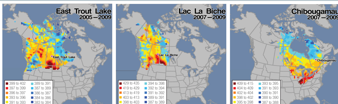
Figure 3. Air flow receptor analysis using measurements of surface CO 2 concentrations (ppm) during the winter months of November to February from the three CCP sites. The site locations are indicated with dots.
